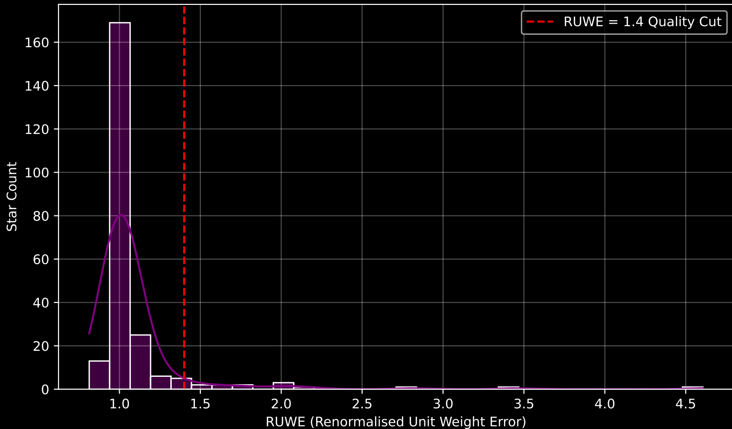
GAPOGEE DR17 Field [M67_btx] RUWE Distribution (n= 231)
