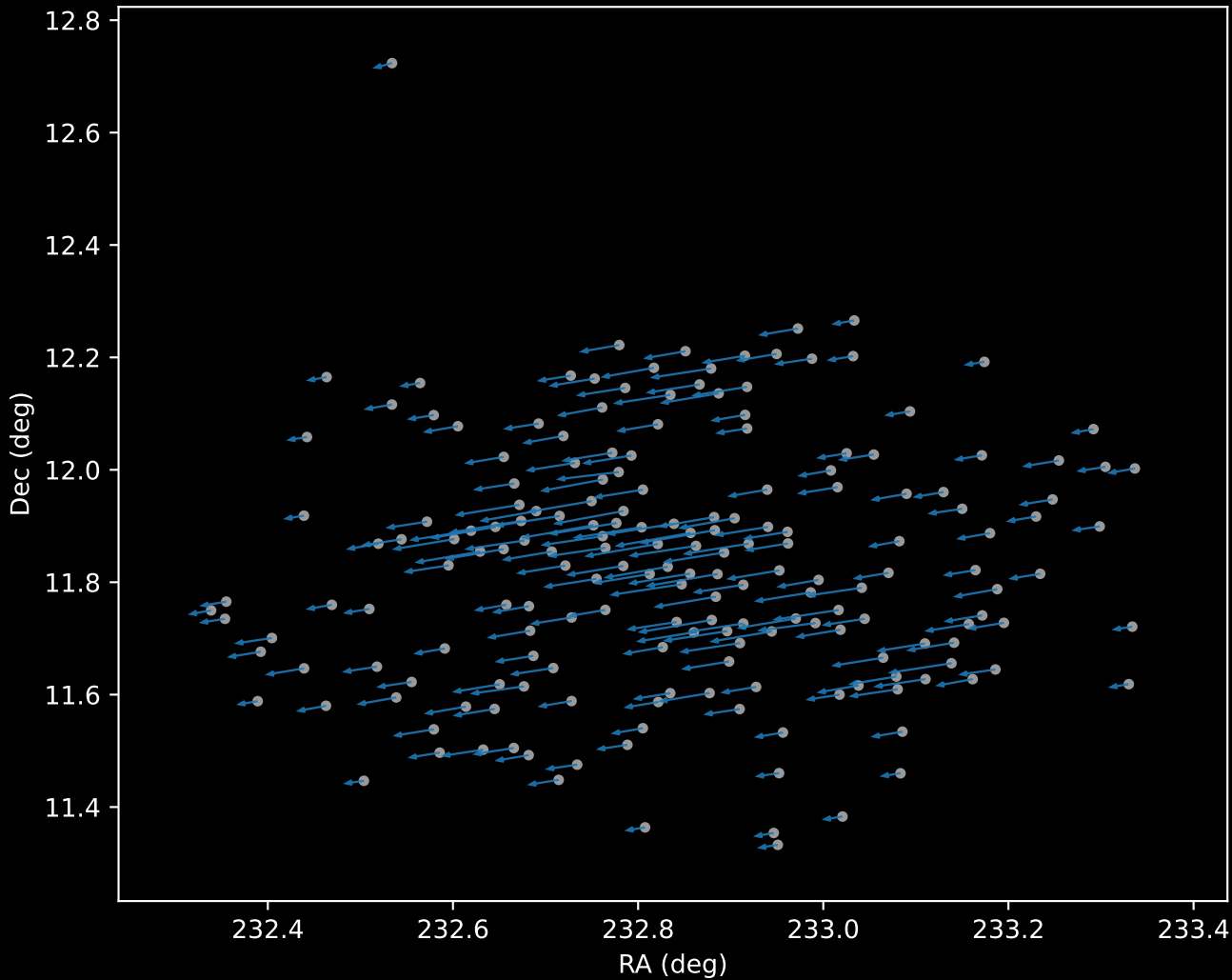
APOGEE DR17 Cluster 0 Proper Motion Vectors (n=190)
