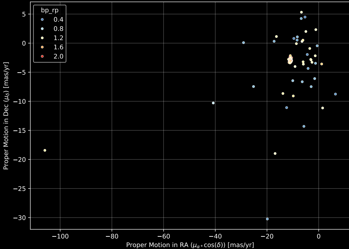
APOGEE DR17 Field: [M67_btx] Proper Motion Diagram (n= 231)
