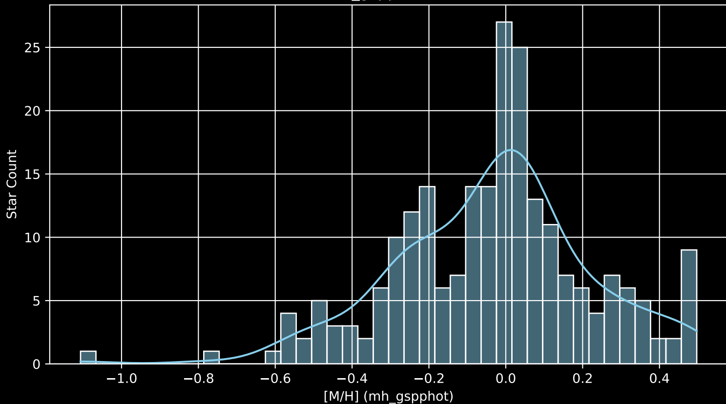
APOGEE DR17 Field: [M67_btx [M/H] (mh_gspphot) (n= 229)
