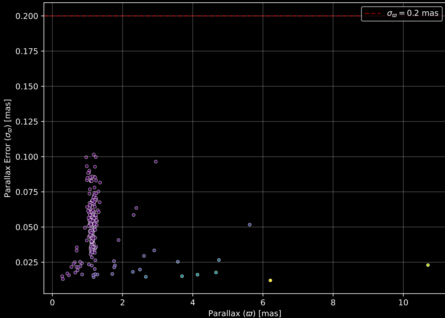
APOGEE DR17 Field: [M67_btx] Parallax Quality (n= 231)
