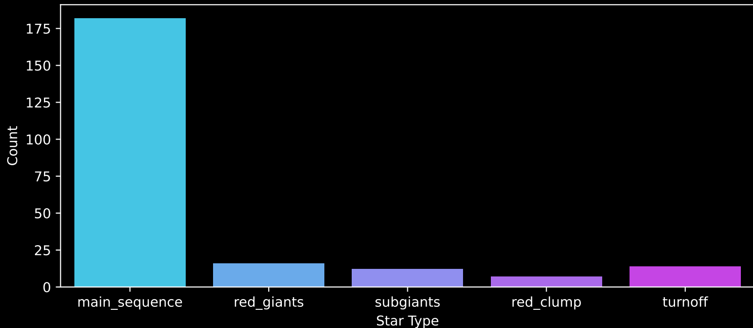
APOGEE DR17 Field: [M67_btx] Count plot of Star Type
